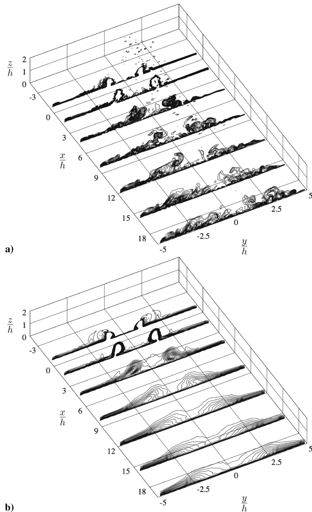
Fig. 5 Streamwise velocity contours for the CFD case in y - z planes along the streamwise direction: a) instantaneous and b) time-averaged. Fourteen contour levels from 0.5 to 0.99 are shown in each plane.
