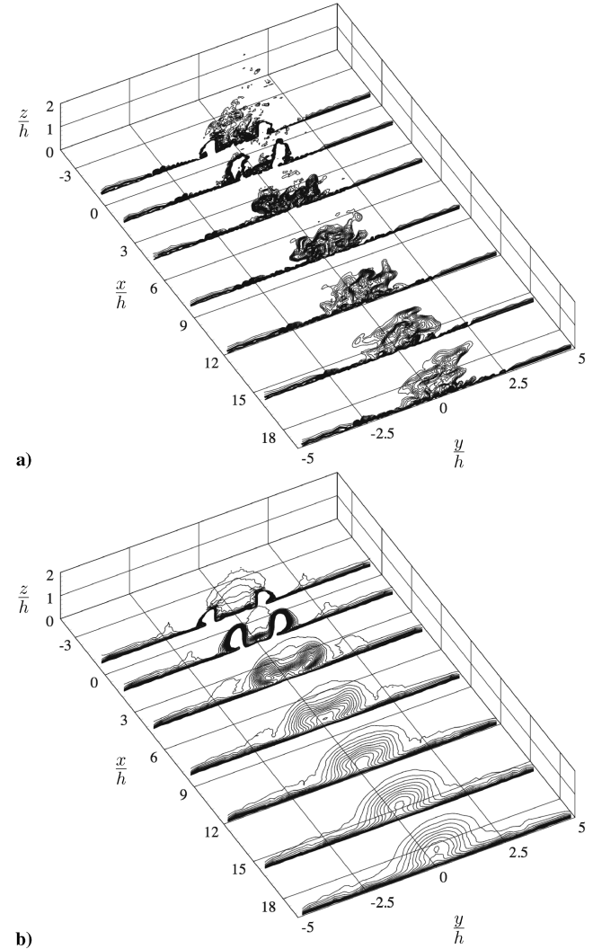
Fig. 6 Streamwise velocity contours for the CFU case in y - z planes along the streamwise direction: a) instantaneous and b) time-averaged. Fourteen contour levels from 0.5 to 0.99 are shown in each plane.
